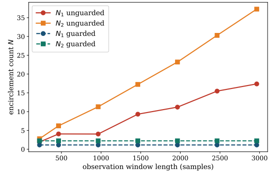
Figure 5: Window dependence of N_1, N_2 on the counterexample plant, guarded (Definition 2) versus unguarded (Definition 1 applied to the raw window). Guarded counts are exactly flat.
