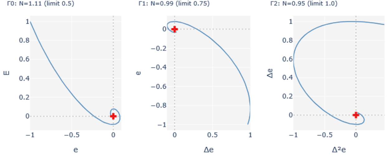
Figure 4: Portraits after tuning. \Gamma_2 is now within its limit (0.95 vs. 1.0); \Gamma_0, \Gamma_1 have fallen sharply from Figure 2 ( 3.75 \rightarrow 1.11 , 4.33 \rightarrow 0.99 ) and sit just outside theirs, the boundary limit cycle of Proposition 7 caught mid-oscillation rather than a rare failure to converge.
