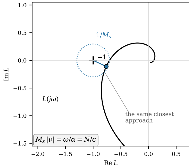
(b) the familiar Nyquist view
