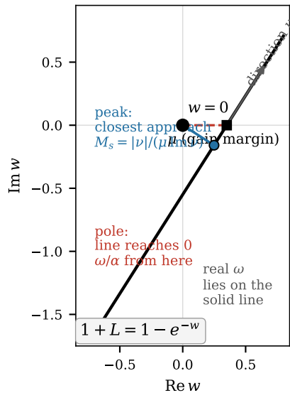
(a) substitute w = \mu + \nu u , u = \ln(\omega/\omega_{180})
