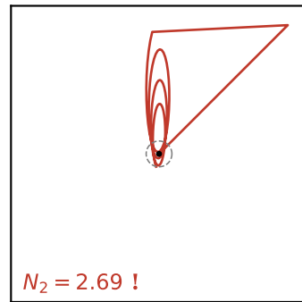
\Gamma_2: (\Delta^2 e, \Delta e)
