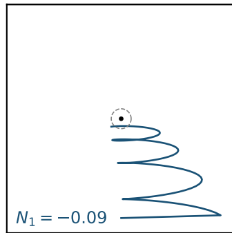
\Gamma_1: (\Delta e, e)
