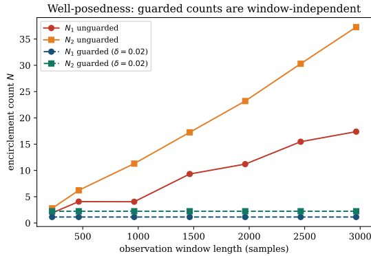
Figure 5: Window dependence of N_1, N_2 on the counterexample plant, guarded (Definition 2) versus unguarded (Definition 1 applied to the raw window). Guarded counts are exactly flat.
