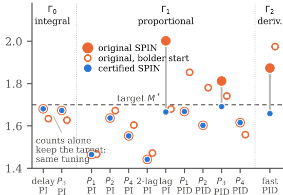
(a) the twelve loops of the table
