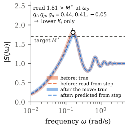
(b) one band move on P_3 with PID
