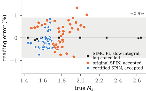
(b) reading error of M_s , every loop
