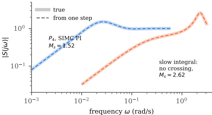
(a) the step gives the whole sensitivity function
