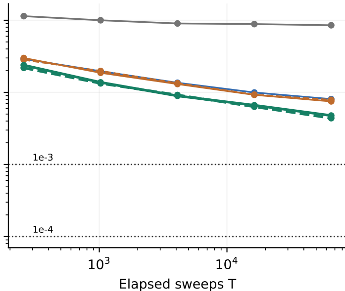
24x24 mixed (576 spins)
