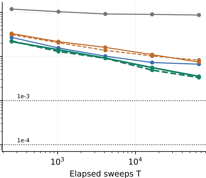
16x16 mixed (256 spins)
