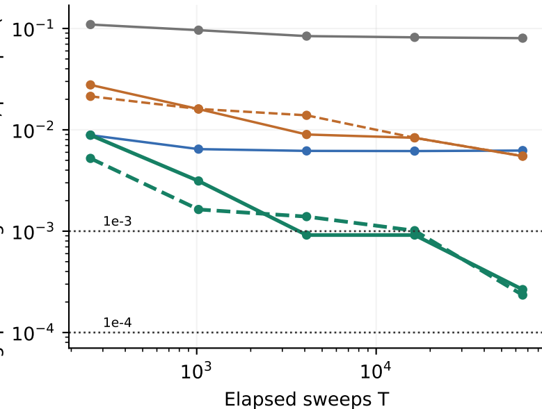
8x8 mixed (64 spins)
