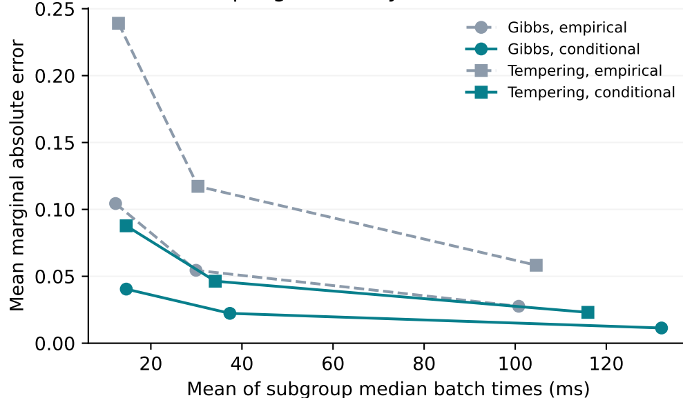
Weak coupling: accuracy versus execution time
