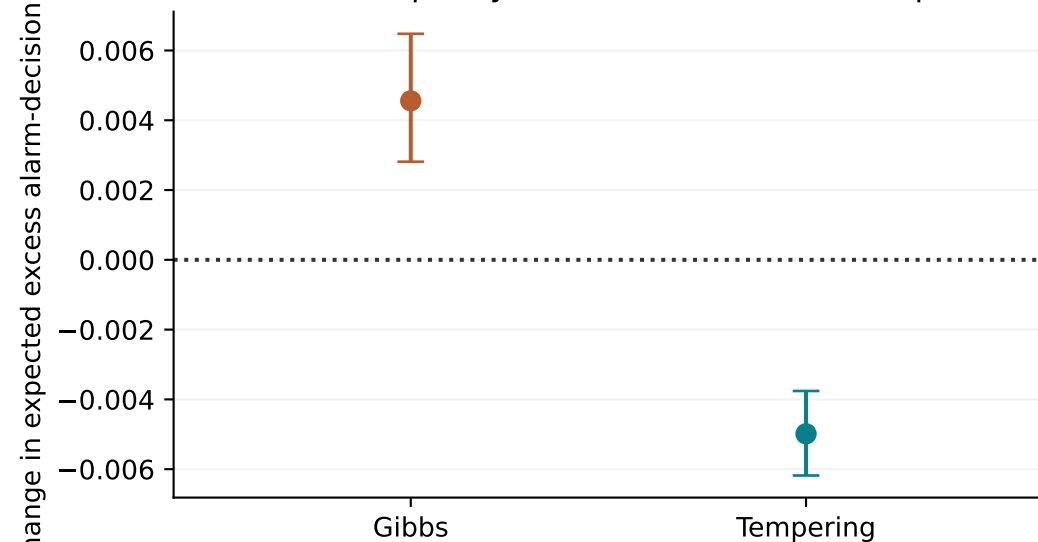
Decision quality: lower is better (16 sweeps)
