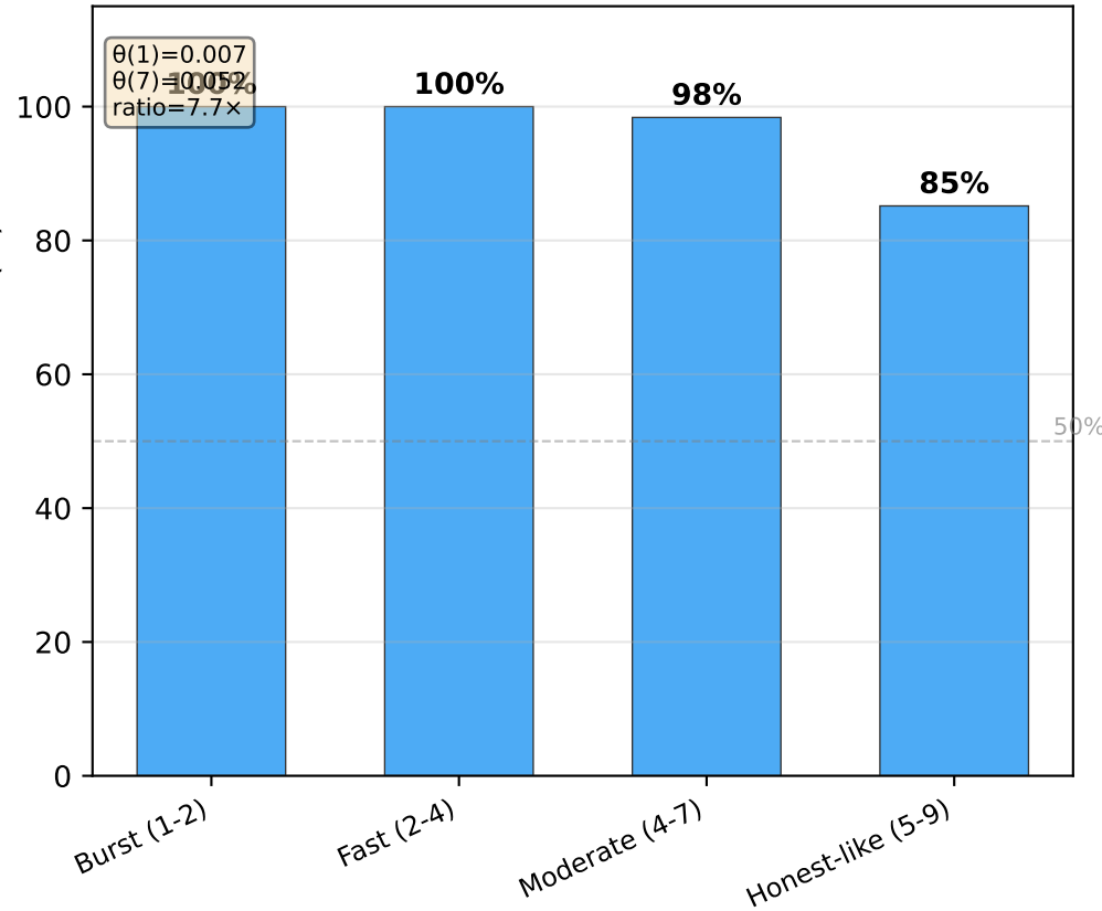
Taktikos LDD (snowplow, f_A=0.5 )
