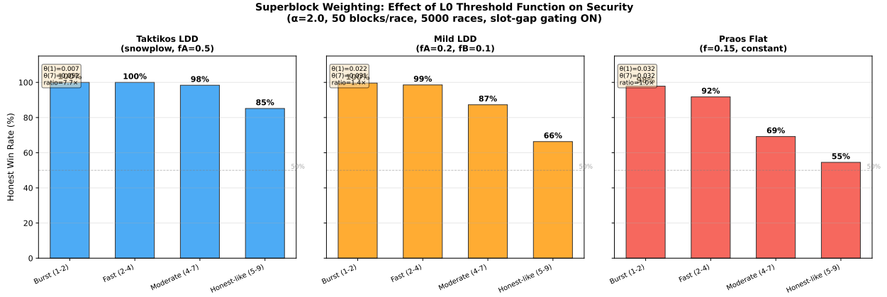
Figure 10: Honest win rates under three L0 threshold functions. Left: Taktikos LDD ( 7.7\times threshold range) achieves near-perfect honest wins across all strategies. Center: Mild LDD ( 1.4\times range) shows erosion at moderate and honest-like gaps. Right: Praos flat ( 1.0\times range, no difficulty gradient) collapses to 69% at moderate gaps—weight-based selection provides only marginal advantage over length-based selection. The 50% line (dashed) represents a fair coin flip.
