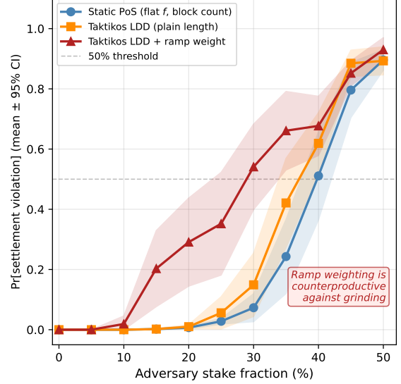
(b) Settlement Security vs. Adversary Stake (grinding simulation, 20 trials per point)
