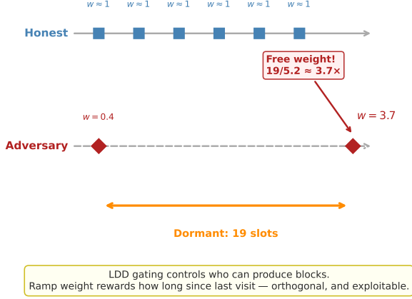
Figure 9: Weighting and grinding resistance. (a) Intuition for why ramp weighting hurts: an adversary’s dormant branch earns high weight (proportional to gap since last visit) when extended, regardless of whether that branch was honestly contested. The LDD election function itself provides the grinding defense—any additional gap-based reward undermines it. (b) Settlement violation probability vs. adversary stake for three schemes (200-fork grinding simulation). Static PoS collapses at \approx 35\% , Taktikos LDD plain collapses at \approx 30\% , while Taktikos LDD + ramp weight collapses at 10%. Ramp weighting is counterproductive against grinding adversaries.
