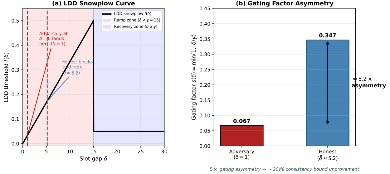
Figure 8: LDD gating asymmetry: the source of consistency improvement. (a) The LDD snowplow threshold curve. Honest blocks (shaded blue band, mean gap \approx 5.2 ) land in the ramp zone; an adversary attempting to maximize block production (gap \delta = 1 , red) is at the bottom of the ramp. (b) The gating factor s(\delta) = \min(1, \delta/\gamma) for honest vs adversary production. The 5\times asymmetry in gating factor translates directly into a \sim 20\% improvement in the consistency bound, independent of the weight function.
