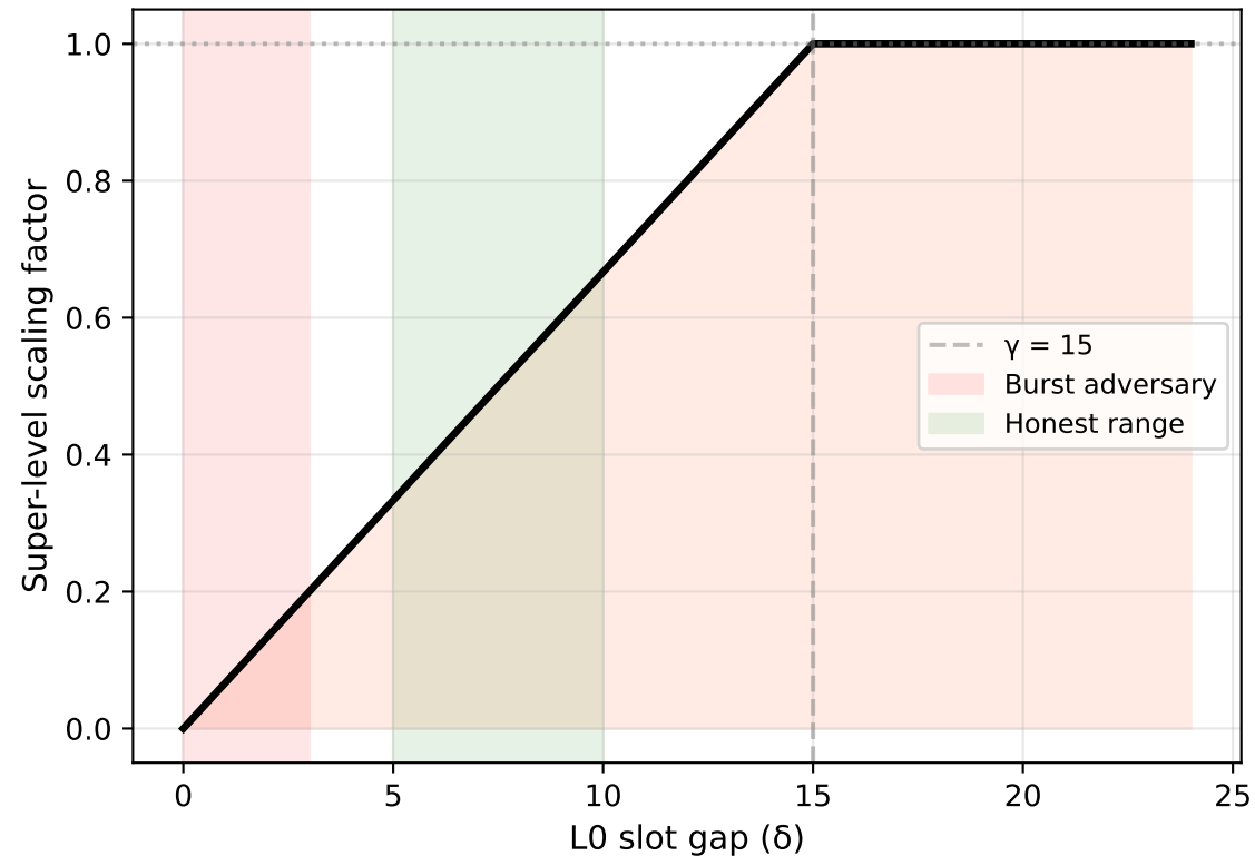
(a) Slot-Gap Scaling: \min(1, \delta/\gamma)
