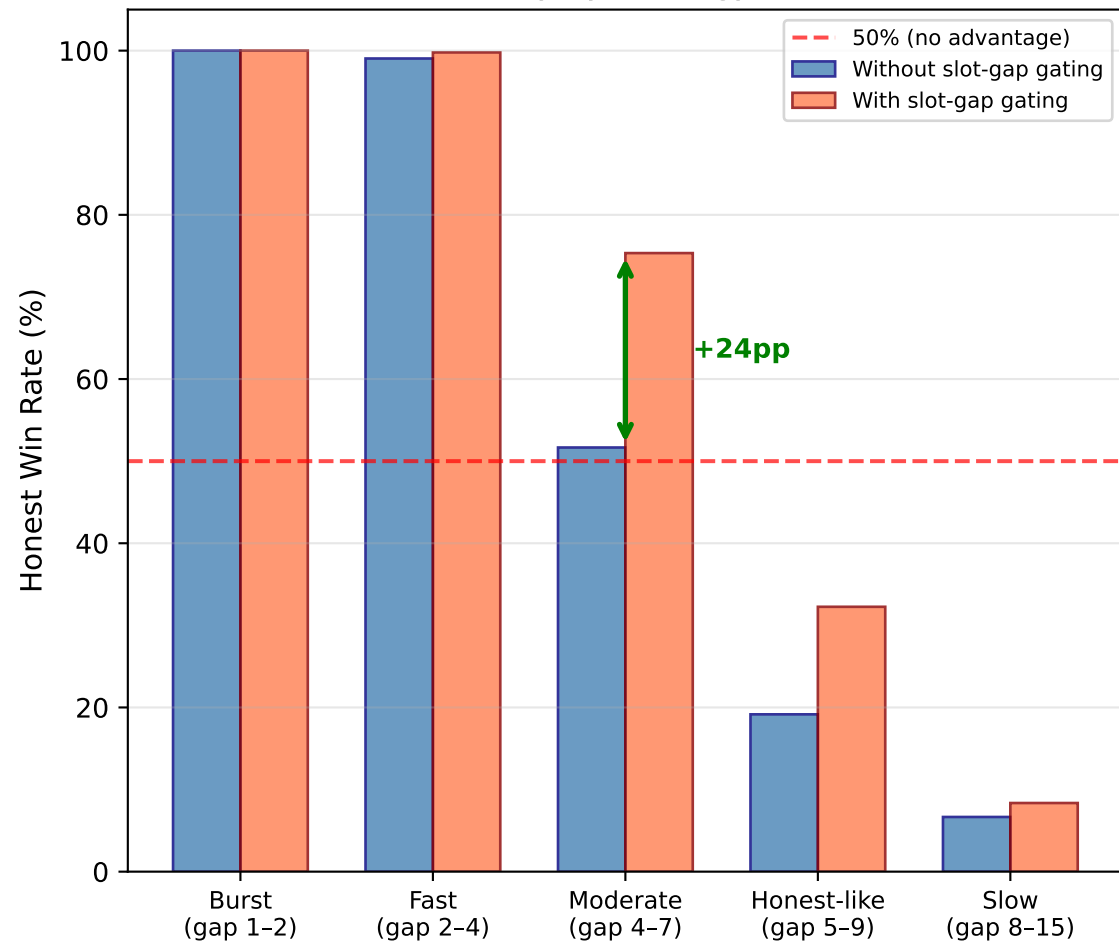
(a) Honest vs Adversary by Strategy ( \alpha = 2.0 , 50 blocks)
