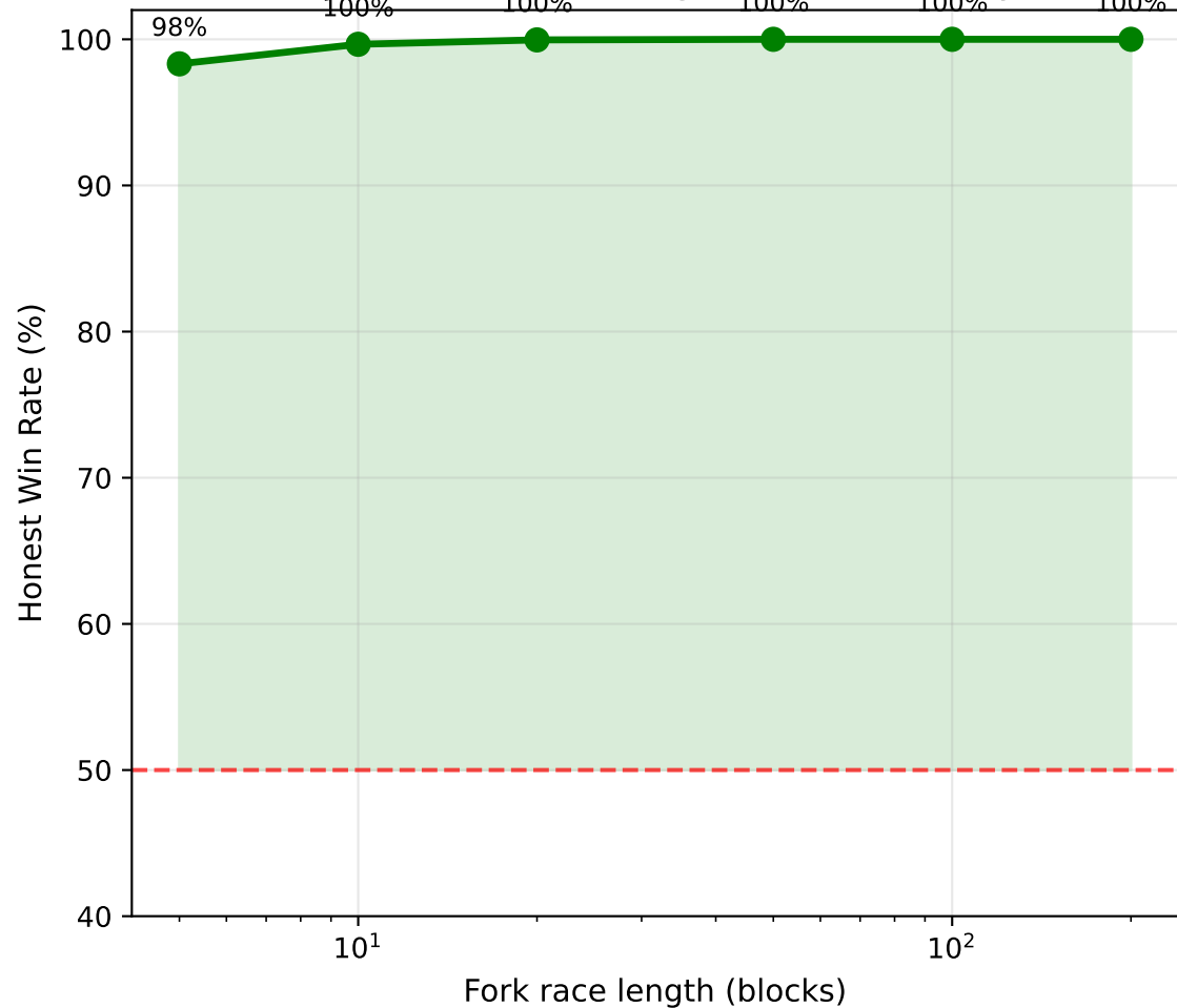
(b) Honest Win Rate vs Fork Length (burst adversary, \alpha = 2.0 )
