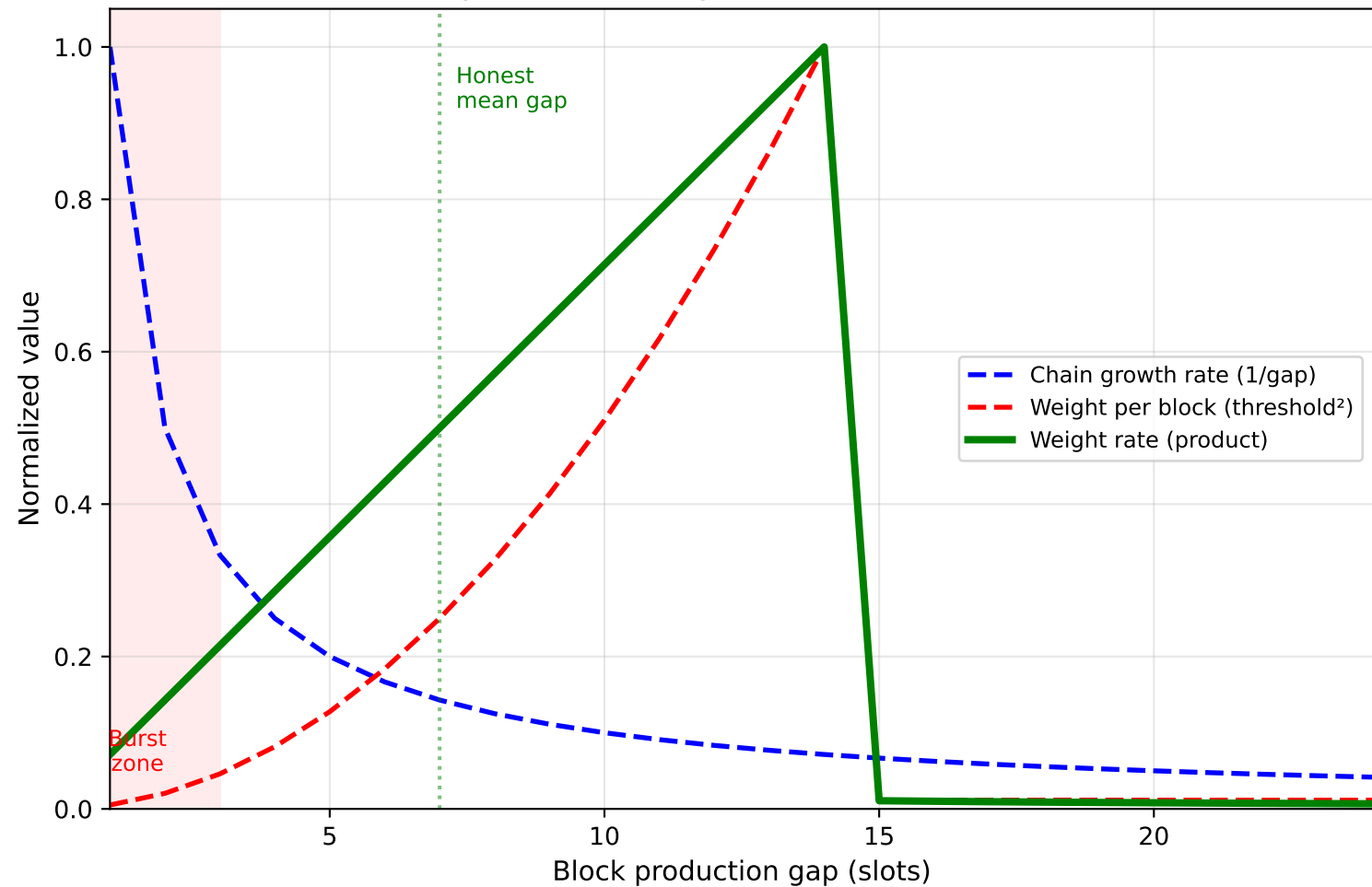
The Adversary Dilemma: Weight Per Block vs Chain Growth Rate
