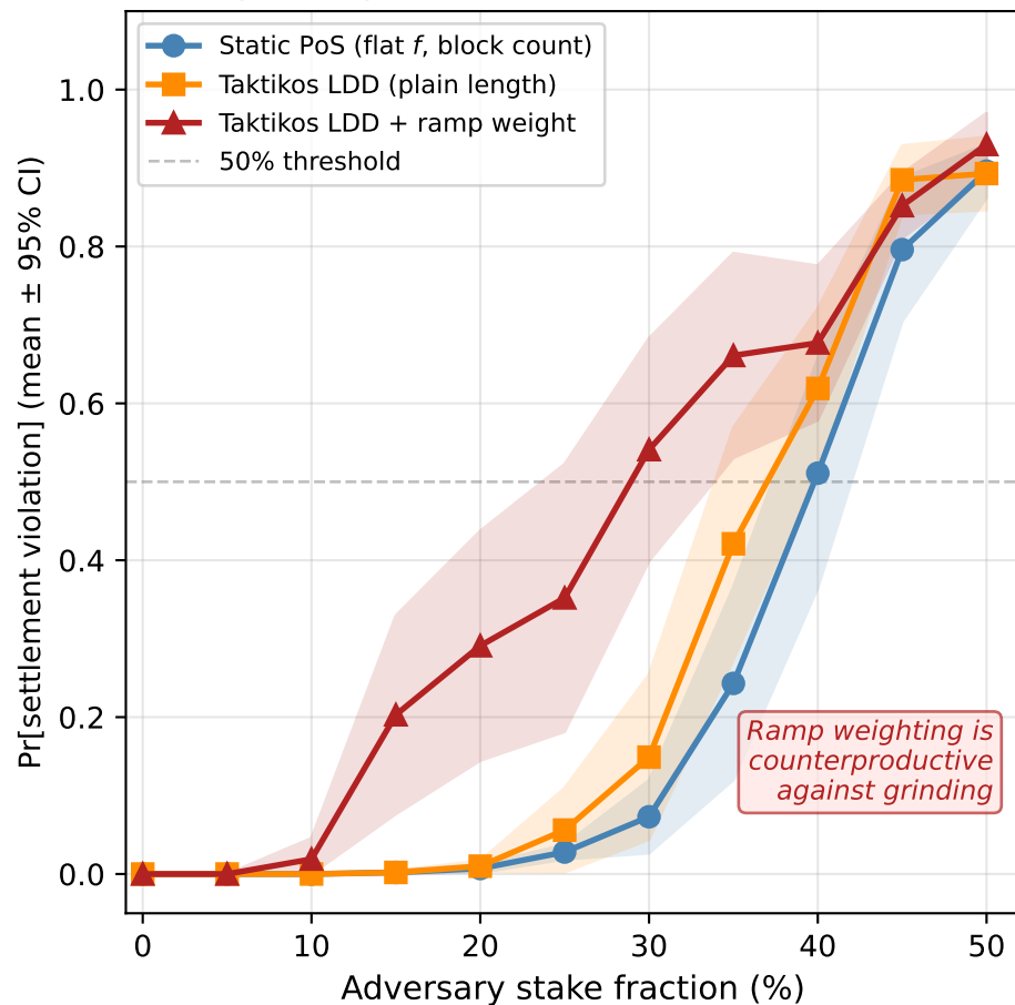
(b) Settlement Security vs. Adversary Stake (grinding simulation, 20 trials per point)
