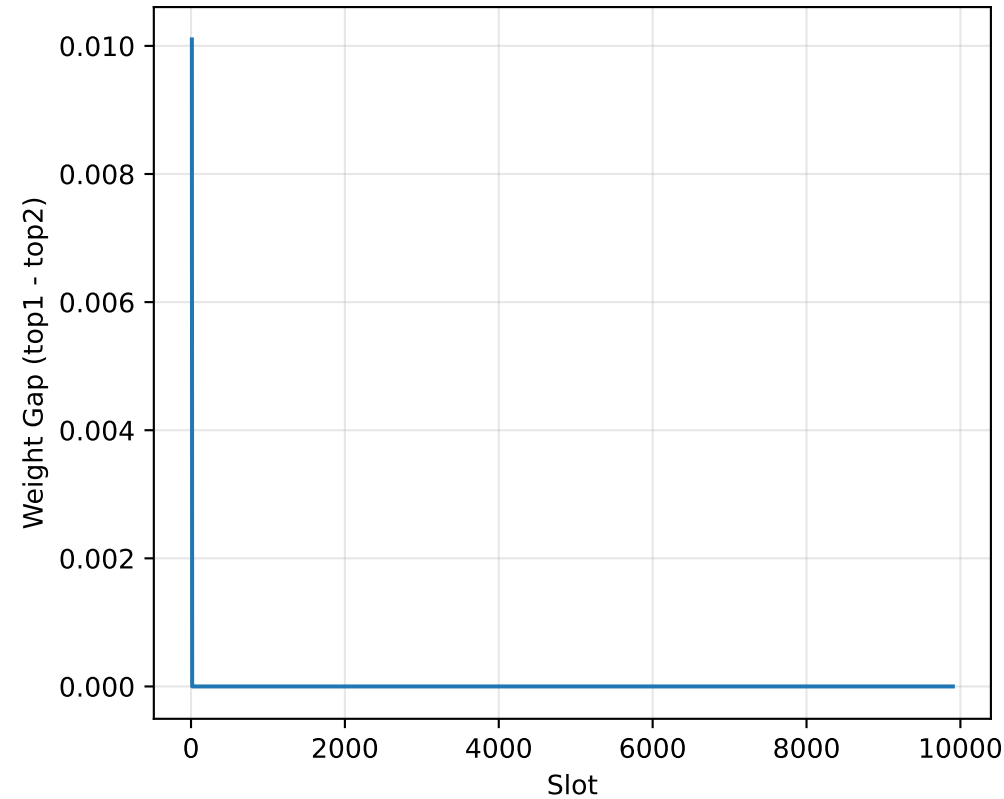
Exponential 3^\mu
