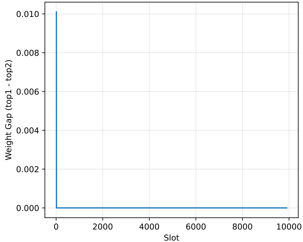
Exponential 2^\mu
