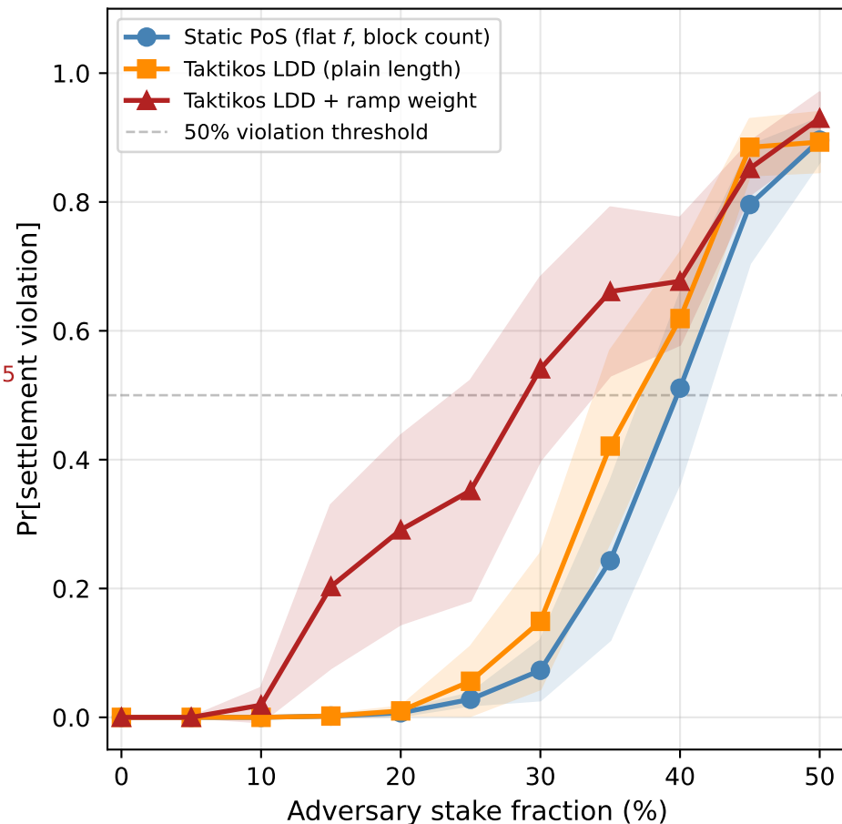
(b) Settlement Security vs. Adversary Stake (50-fork grinding sim, N = 20 trials, shading = 95% CI)
