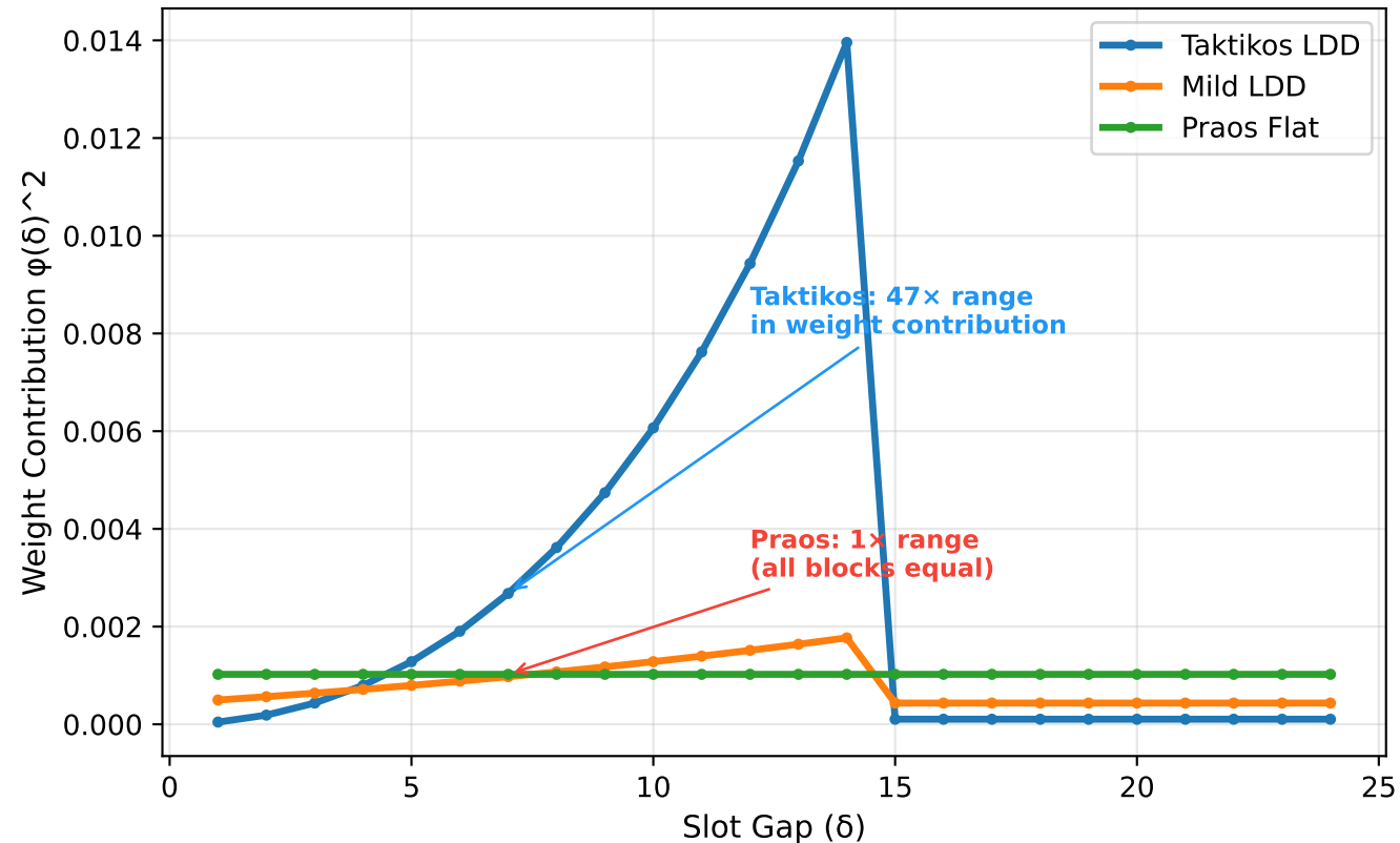
L0 Weight Component ( \alpha=2 )
