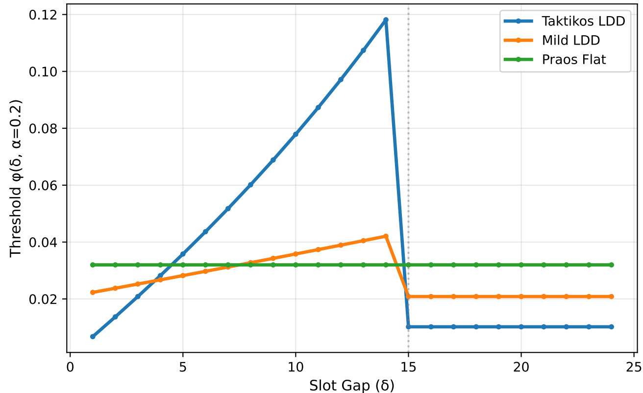
L0 Threshold Functions
