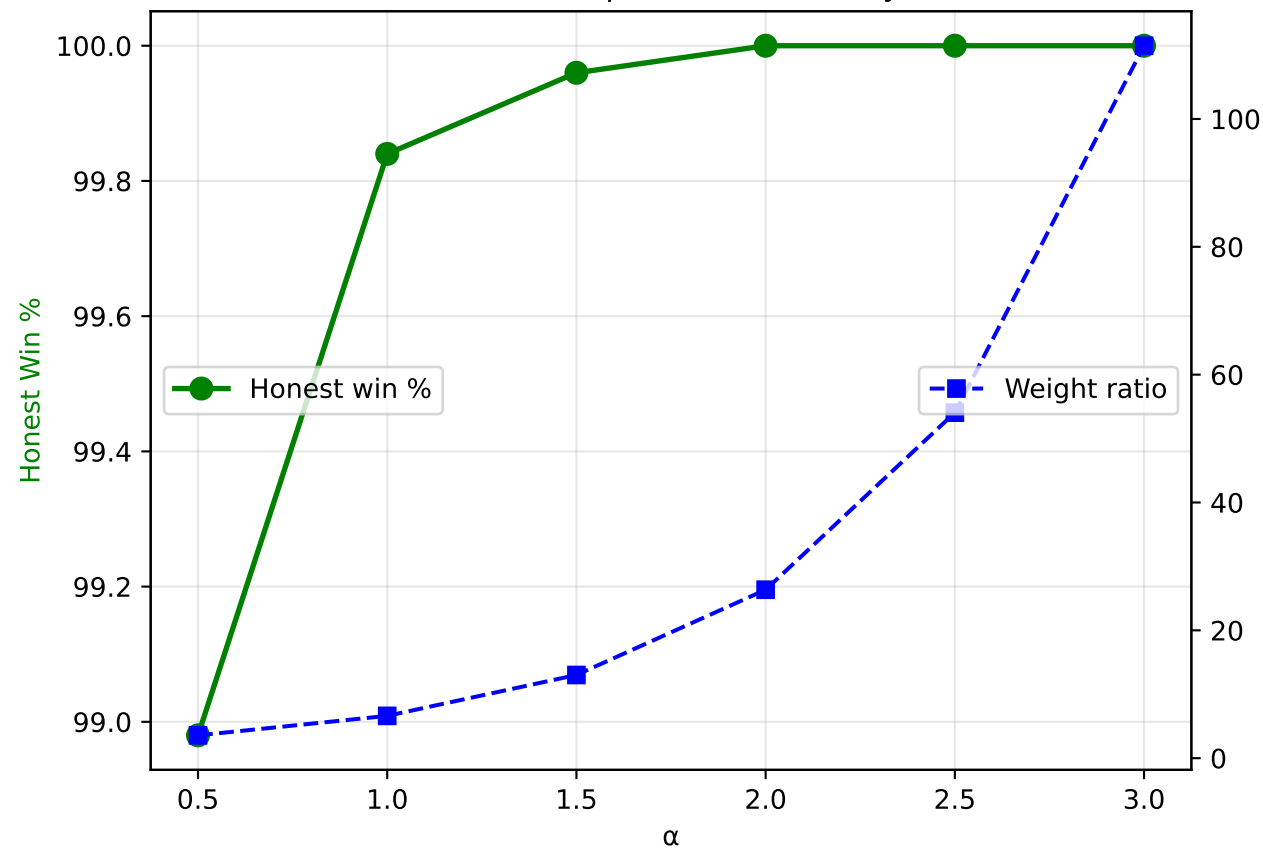
v3: \alpha Sweep (burst adversary)
