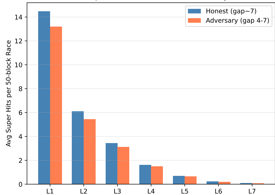
v3: Super Hit Rates (moderate adversary)
