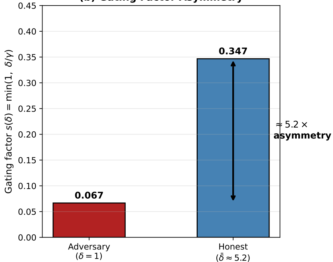
(b) Gating Factor Asymmetry
