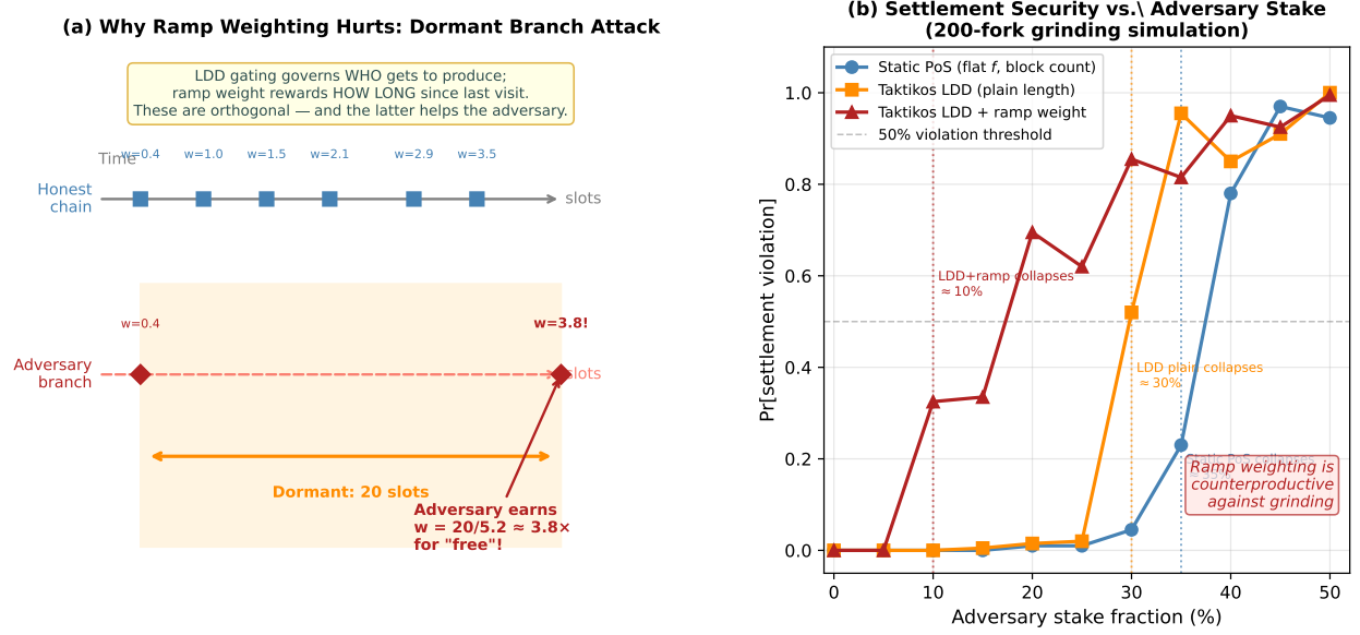
Figure 9: Weighting and grinding resistance. (a) Intuition for why ramp weighting hurts: an adversary’s dormant branch earns high weight (proportional to gap since last visit) when extended, regardless of whether that branch was honestly contested. The LDD election function itself provides the grinding defense—any additional gap-based reward undermines it. (b) Settlement violation probability vs. adversary stake for three schemes (200-fork grinding simulation). Static PoS collapses at \approx 35\% , Taktikos LDD plain collapses at \approx 30\% , while Taktikos LDD + ramp weight collapses at 10\% . Ramp weighting is counterproductive against grinding adversaries.
