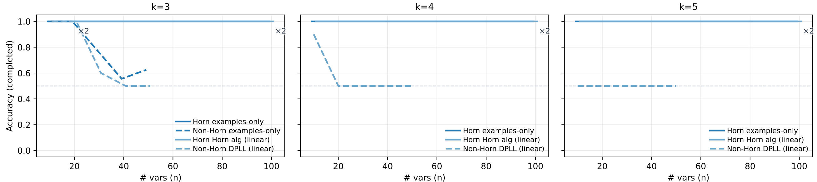
Prompting-policy effects (OpenAI · gpt-5.2-pro · think=high · Compact CNF)
