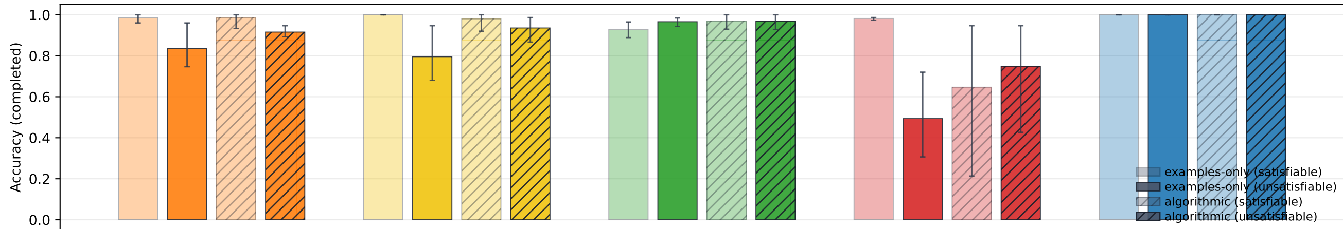
Horn subset
