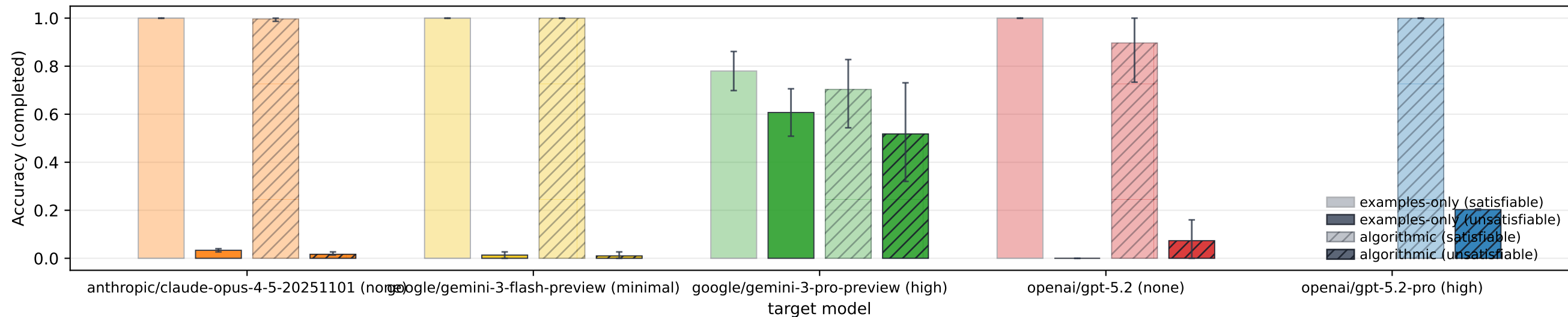
Non-Horn subset
