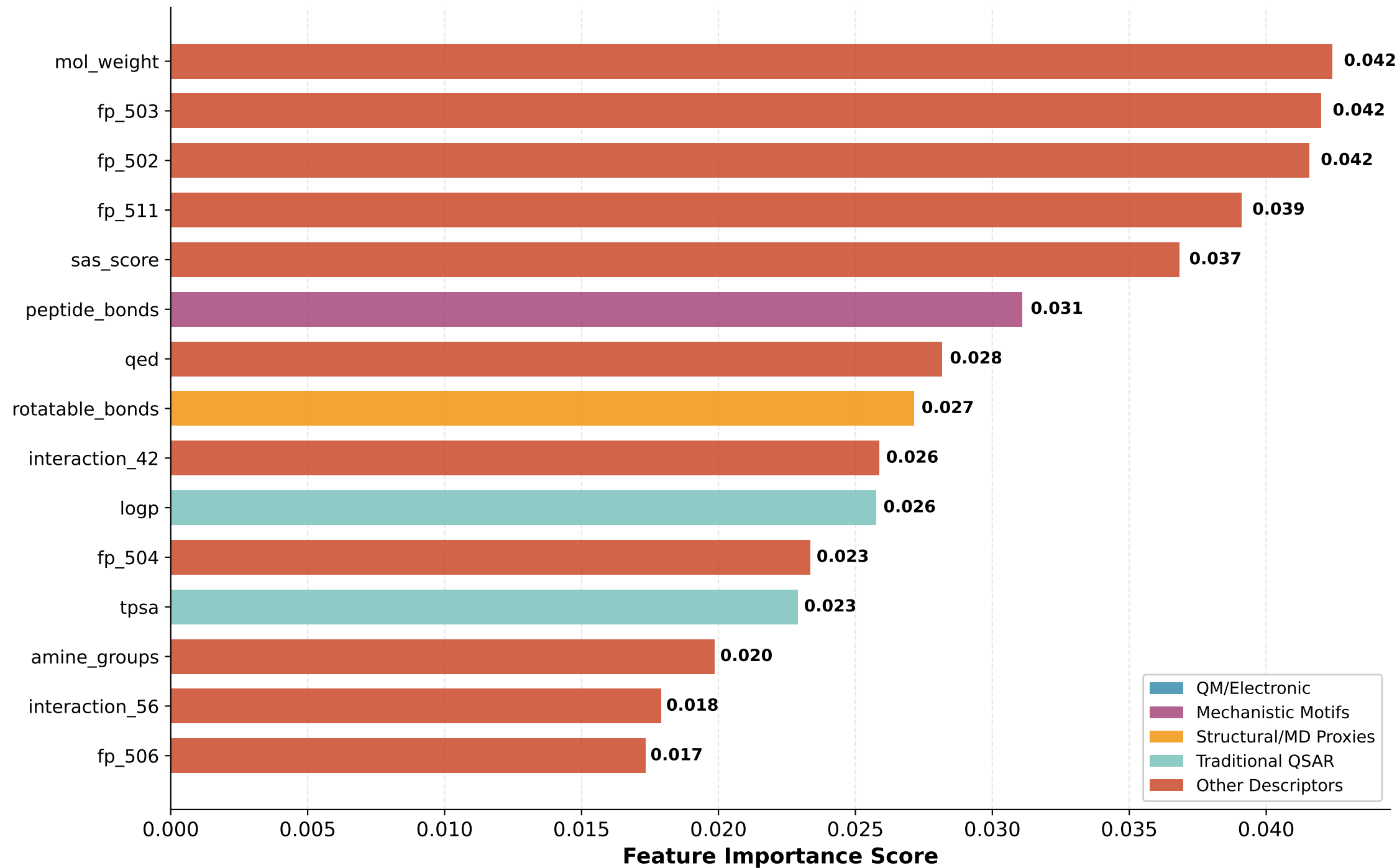
Top 15 Most Important Features in Multi-Modal Model
