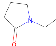
PVP (fragment) -2101.6 kJ/mol
