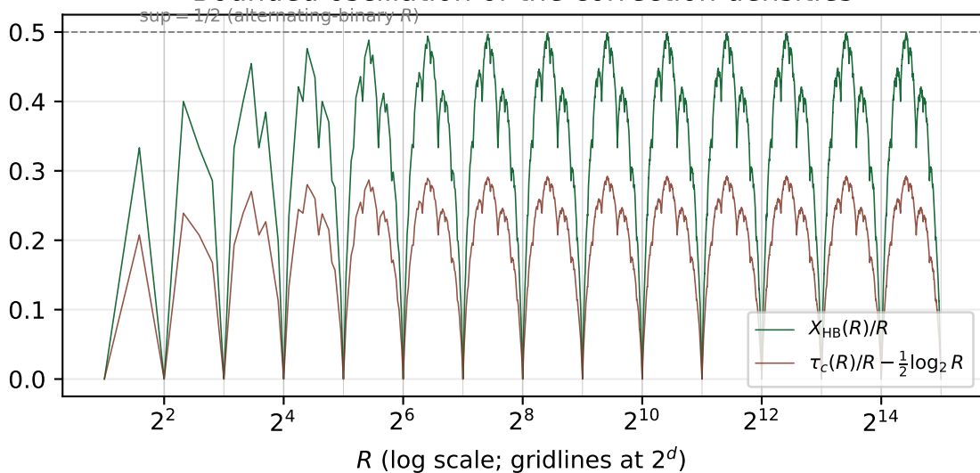
Bounded oscillation of the correction densities
