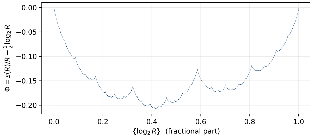
Delange fluctuation \Phi(\log_2 R) of s(R) (A000788)
