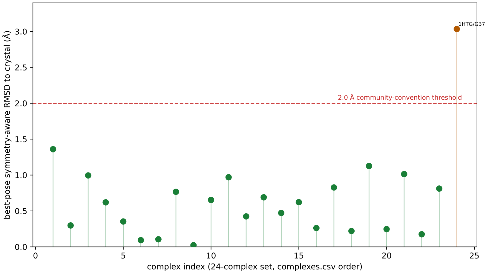
Redocking benchmark: 23/24 complexes within 2.0 Å (best-any-rank; 95% CI 79.8–99.3%)
