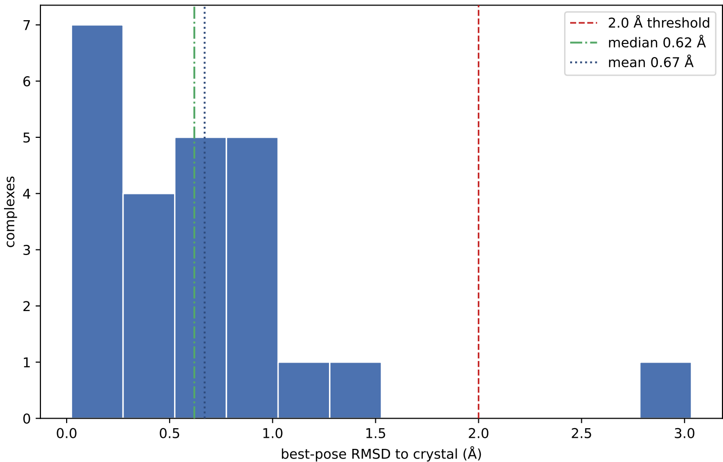
RMSD distribution (n=24); success 23/24 = 95.8% (95% Wilson CI 79.8–99.3%)
