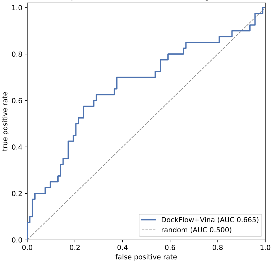
DUD-E hivpr enrichment evaluation (133 ligands, exh. 1)
