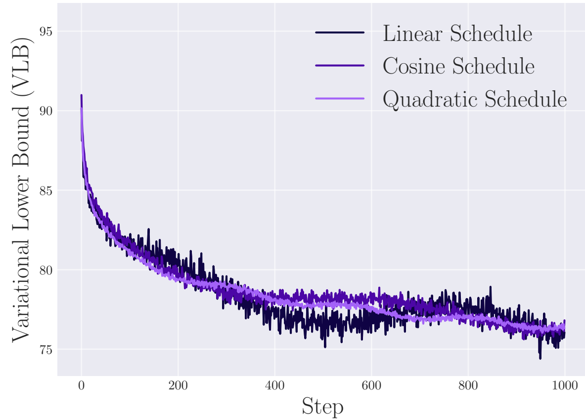
CIFAR-10
