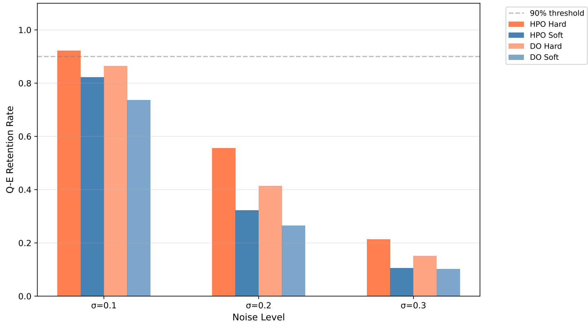
Q-E Retrieval Retention Under Noise (Baseline = 100%)
