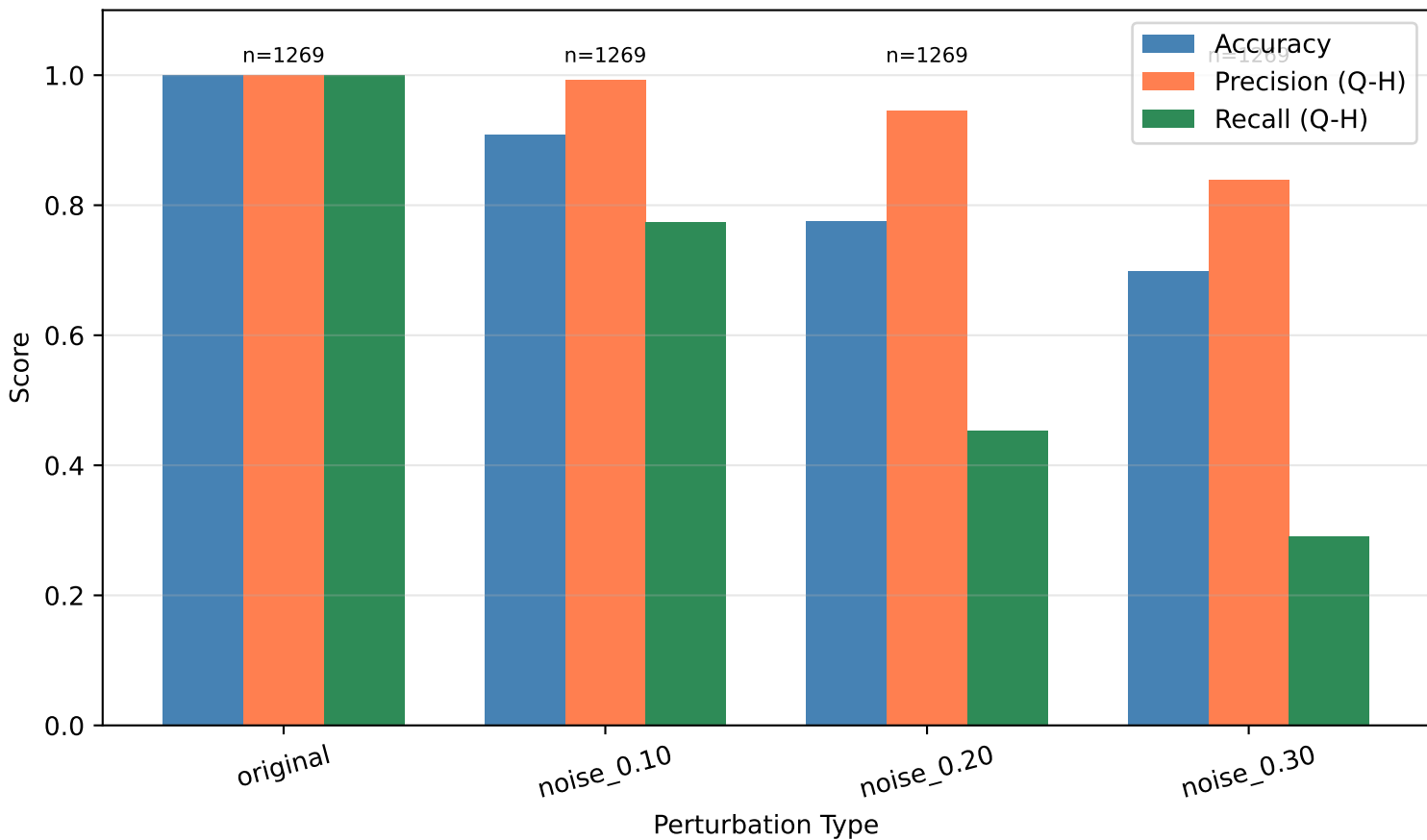
Gate Robustness Test: HPO
