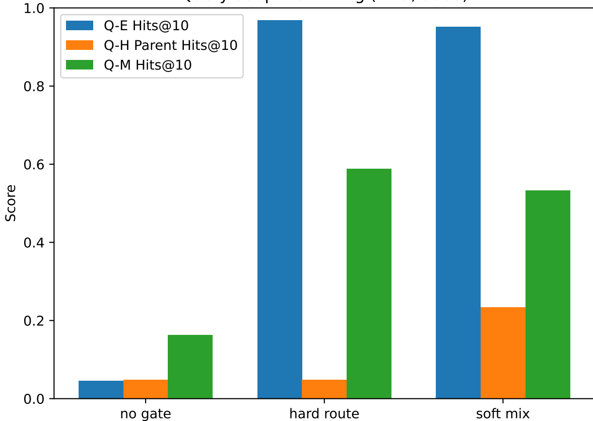
Query-adaptive mixing (HPO, 5000)
