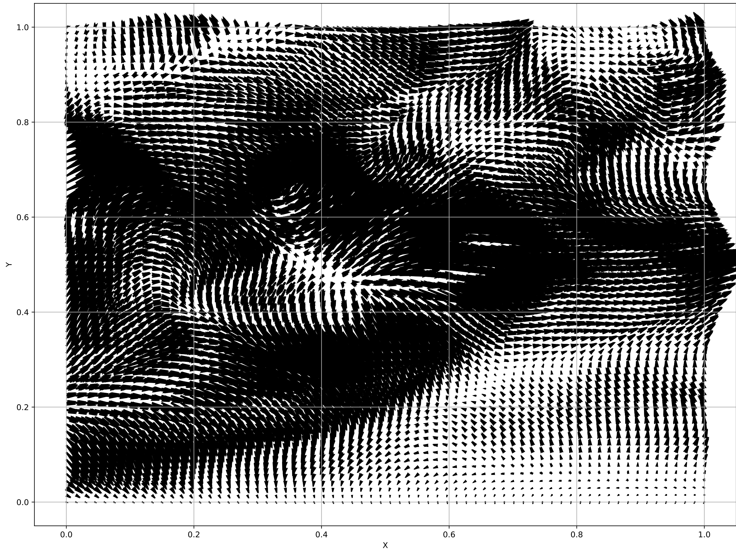
Mean Wind Vector Field
