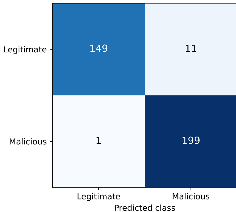
Logistic Regression
