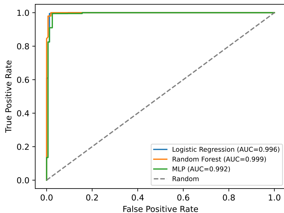
ROC Curves
