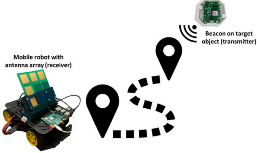
Figure 7: Configuration of proposed setup of Bluetooth homing controller.
