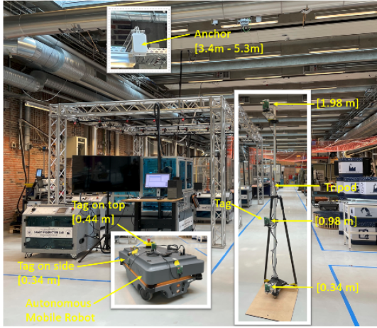
Figure 9: UWB anchor-tag geometry for ranging and multilateration-based localization in indoor environments.
