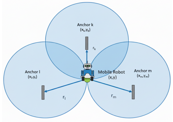
Figure 10: Illustration of multilateration technique. Each known anchor forms a circle with radius equal to its distance to the robot, and the robot's estimated position is where these circles intersect.
