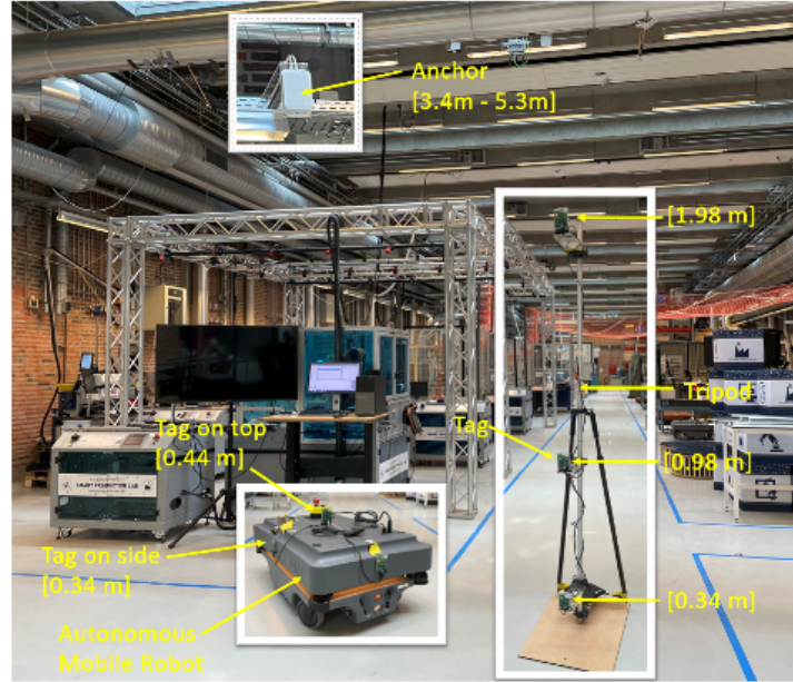
Figure 8: UWB anchor-tag geometry for ranging and multilateration-based localization in indoor environments.
