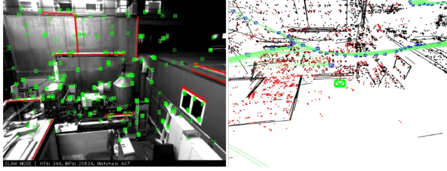
Figure 10: Illustration of SLAM fusion: visual/laser perception integrated with inertial and odometric constraints for robust state estimation.
