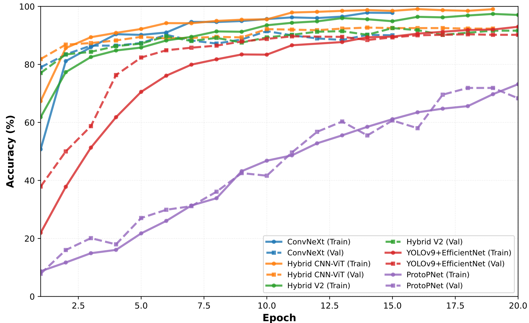
Training and Validation Accuracy Over Epochs
