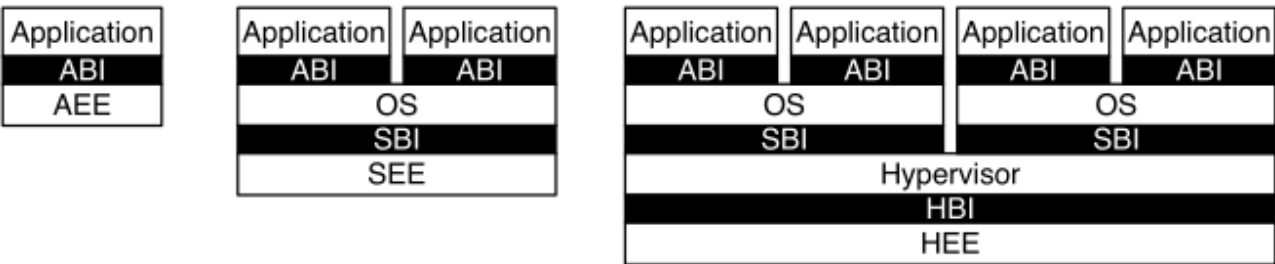
Figure 8. Different implementation stacks supporting various forms of privileged execution.
