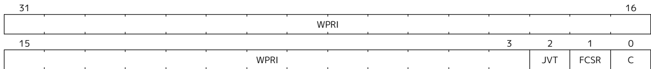
Figure 118. Supervisor State Enable 0 Register ( sstateen0 )
