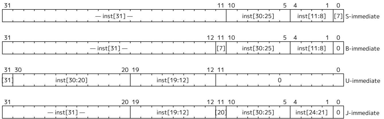
Figure 1. Types of immediate produced by RISC-V instructions.
