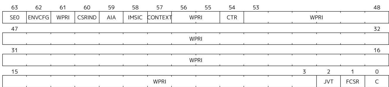
Figure 117. Hypervisor State Enable 0 Register ( hstateen0 )
