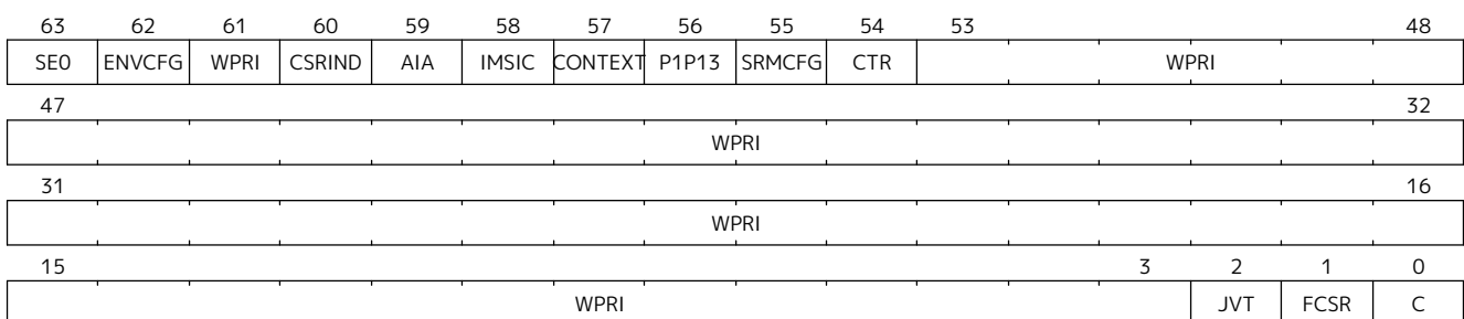
Figure 116. Machine State Enable 0 Register ( mstateen0 )
