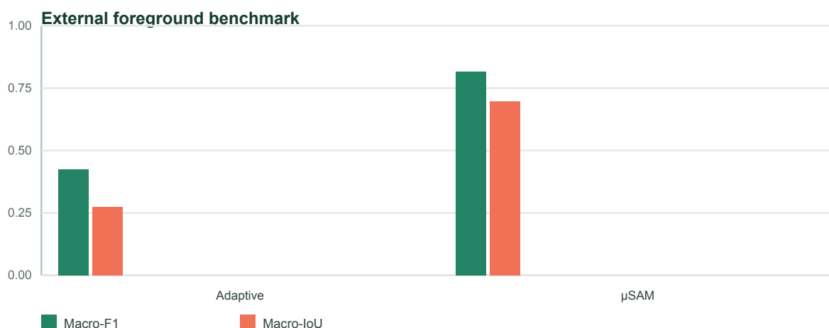
Figure 2. BBBC019 macro scores; the stronger \mu SAM result carries much higher measured cost.
