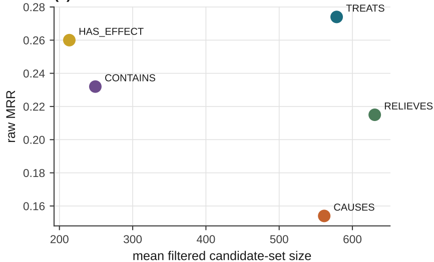
(a) Raw MRR tracks candidate-set size
