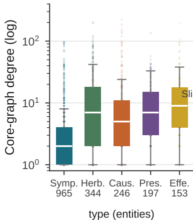
Degree by entity type
