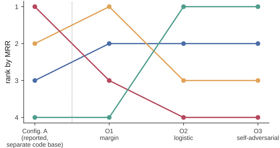
(b) The ordering follows the objective
