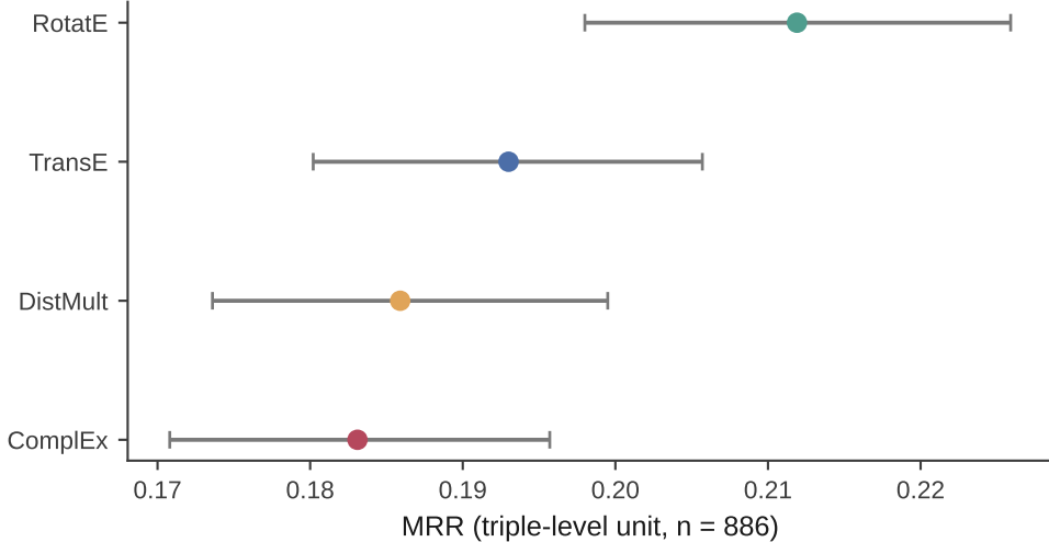
(c) Cluster-bootstrap intervals overlap
