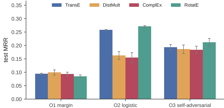
(a) One code base, three objectives (60 epochs)
