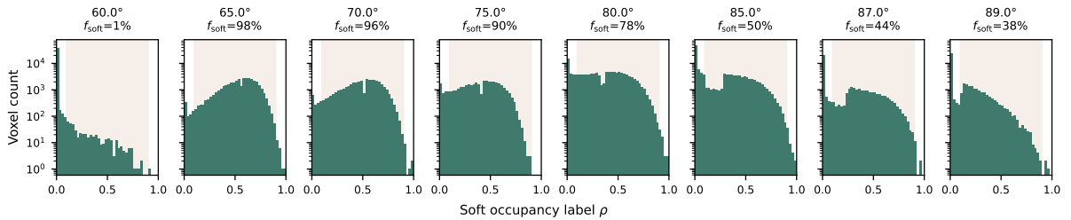
Figure 6: Table 4’s f_{\text{soft}} column is not an artefact of binning choice: at every angle except 60^\circ , most of the voxel mass visibly sits in the ambiguous band rather than piling up at 0 or 1. Distribution of the soft occupancy label \rho_{\text{vox}} on the training split, per deposition angle (log-scale voxel count). Shaded band: the ambiguous range \rho_{\text{vox}} \in (0.1, 0.9) used to define f_{\text{soft}} . At \alpha = 60^\circ almost all voxels sit near \rho_{\text{vox}} = 0 (empty), giving a clean, learnable binary signal; from \alpha = 65^\circ onward, the distribution broadens into the shaded band and a binary classifier has little unambiguous signal left to fit, exactly the effect discussed below.
