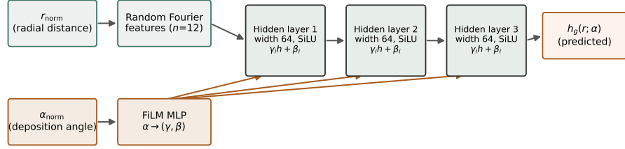
FiLM: each hidden layer's activation is rescaled by \gamma_i(\alpha) and shifted by \beta_i(\alpha) before the nonlinearity — the network's function of r changes continuously with \alpha , the same way a parametric dispersion model is evaluated at any wavelength without refitting.
