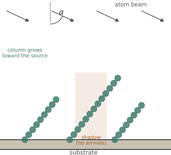
(a) Ballistic shadowing, side view
