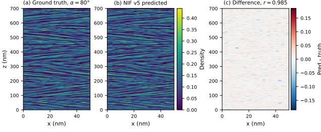
FIG. 3. The high Pearson correlation in Table I is not a coincidence of a coarse aggregate statistic: the network reproduces the fine, tilted-column texture of the ground-truth field directly, and the residual is visually featureless. Vertical ( xz ) slice through the trained NIF v5 field at \alpha = 80^\circ (a training angle), generated by a single forward pass through the saved checkpoint (no retraining). (a) Ground-truth density field. (b) NIF v5 prediction. (c) Pointwise difference (predicted – truth); r = 0.985 for this slice, consistent with Table I.
