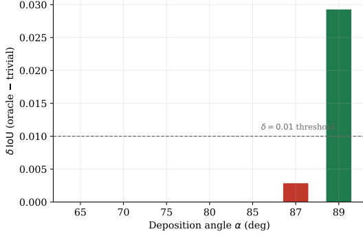
FIG. 5. Independently reproduced from the archived dataset (see provenance note, Section III C): a predictor given the best possible depth information (and no lateral spatial reasoning at all) does not beat the trivial guess, suggesting the missing signal may not be something a better architecture alone could recover from these labels. \delta\text{IoU} (oracle minus trivial) per deposition angle. The oracle uses depth information ( z ) in addition to \alpha ; any positive \delta\text{IoU} would indicate a learnable depth signal in the soft labels. Dashed line: \delta = 0.01 significance threshold. All main production alphas ( 65^\circ – 87^\circ ) fall below this threshold, consistent with depth adding no actionable binary boundary information in the max-normalised soft labels.
