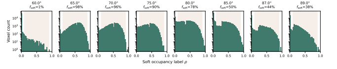
FIG. 6. Table III’s f_{\text{soft}} column is not an artefact of binning choice: at every angle except 60^\circ , most of the voxel mass visibly sits in the ambiguous band rather than piling up at 0 or 1. Distribution of the soft occupancy label \rho_{\text{vox}} on the training split, per deposition angle (log-scale voxel count). Shaded band: the ambiguous range \rho_{\text{vox}} \in (0.1, 0.9) used to define f_{\text{soft}} . At \alpha = 60^\circ almost all voxels sit near \rho_{\text{vox}} = 0 (empty), giving a clean, learnable binary signal; from \alpha = 65^\circ onward, the distribution broadens into the shaded band and a binary classifier has little unambiguous signal left to fit, exactly the effect discussed below.
