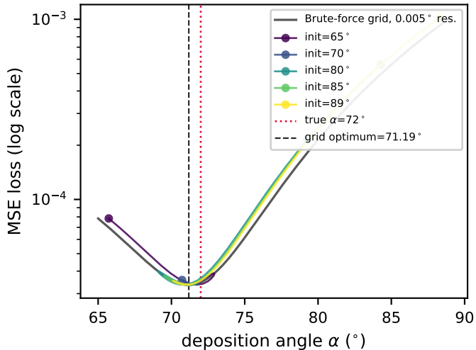
(a) loss landscape + gradient trajectories
