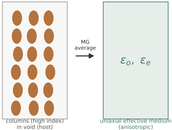
(a) Real geometry \rightarrow effective medium
