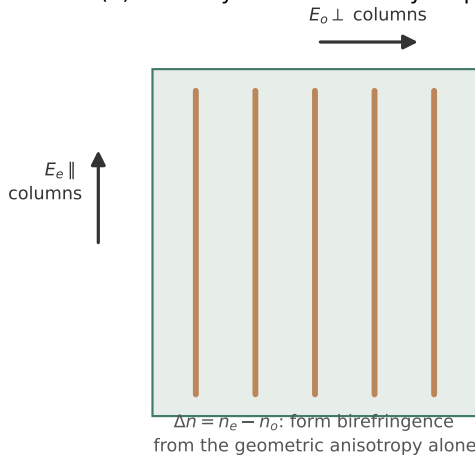
(b) Ordinary vs extraordinary response
