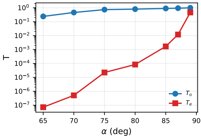
Beer-Lambert transmission
