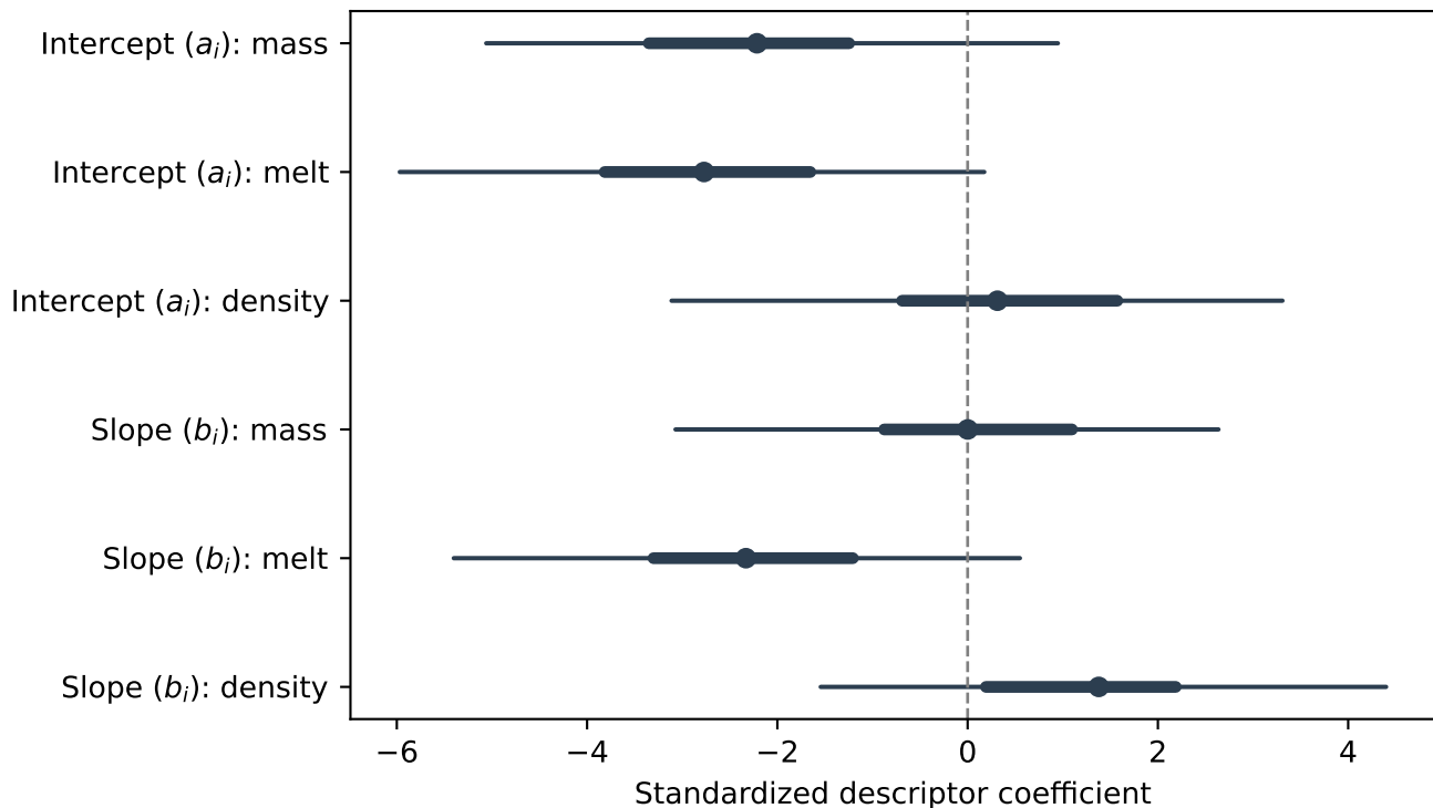
Bayesian hierarchical model: population-level descriptor coefficient (n=250 rows, 46 materials; dots = mean, thick/thin bars = 50%/94%)
